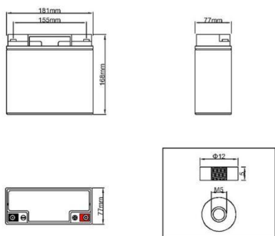
12V17Ah
