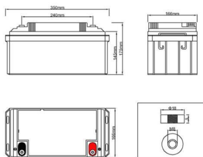
12V65Ah
