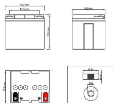
12V38Ah
