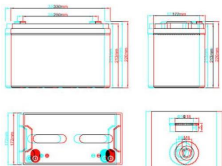
12V100Ah
