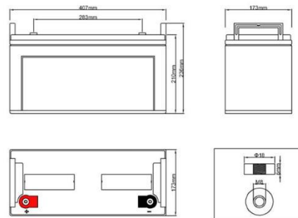
12V120Ah
